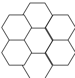
Fig 1.Hexagonal Structure
